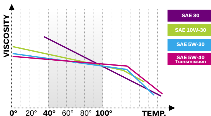
Viscosity performance
