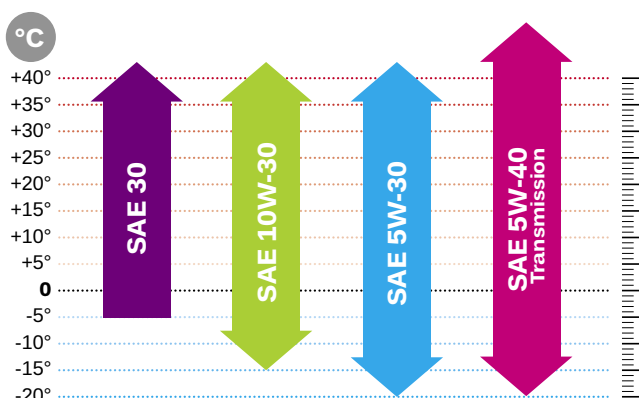
Temperature performance
